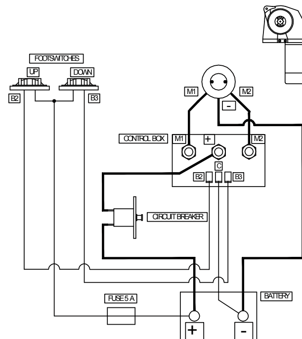
3 Terminals Motors
